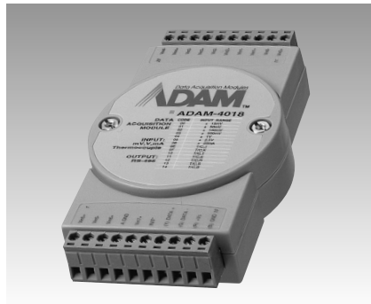
ADAM-4018/4018+
